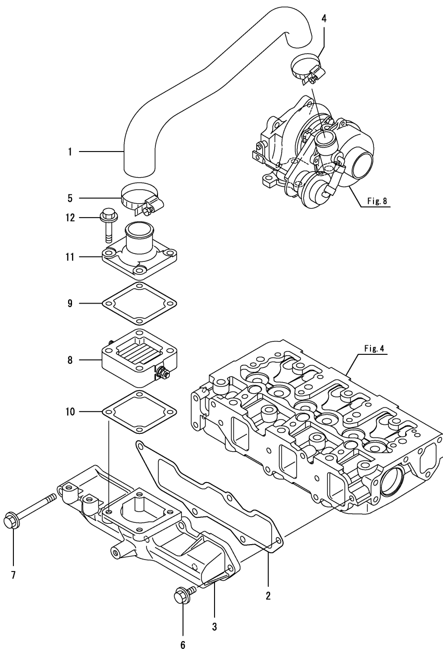
Fig.5. SUCTION MANIFOLD
